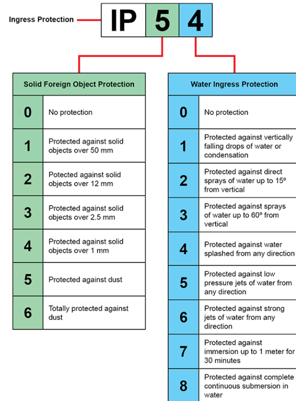
Ingress Protection (IP) Ratings Chart
